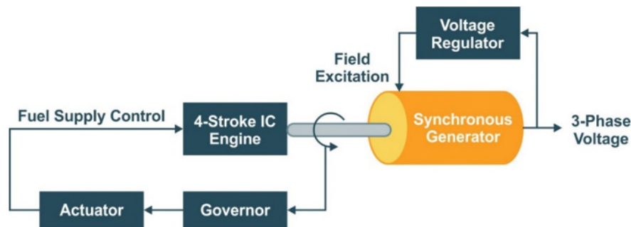
Figure 2: Diesel Generator Parts
